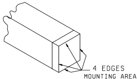
FIGURE 3. Mounting area.
